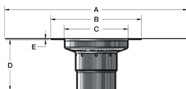
Stainless steel 50 mm (2") no-hub outlet
