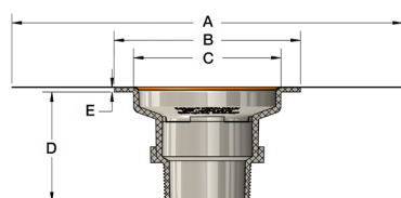
Polypropylene 50 mm (2") outlet
