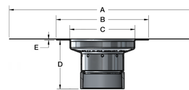
Stainless steel 50 mm (2") threaded outlet
