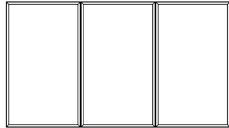
Example: Ganging Mirror-to-Cabinet Arrangement Note: One Mirror Ganging Kit is required per mirror. Reference the Profiles PMGKIT Specification sheet for details
