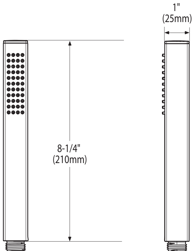
CRITICAL DIMENSIONS (DO NOT SCALE)
