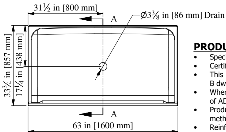
PLAN 63" [1600mm] Barrier-Free Shower w/ 3/4" [19mm] Threshold
